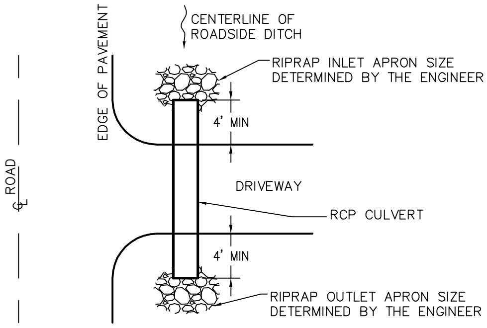
TYPICAL DRIVEWAY PLAN VIEW
