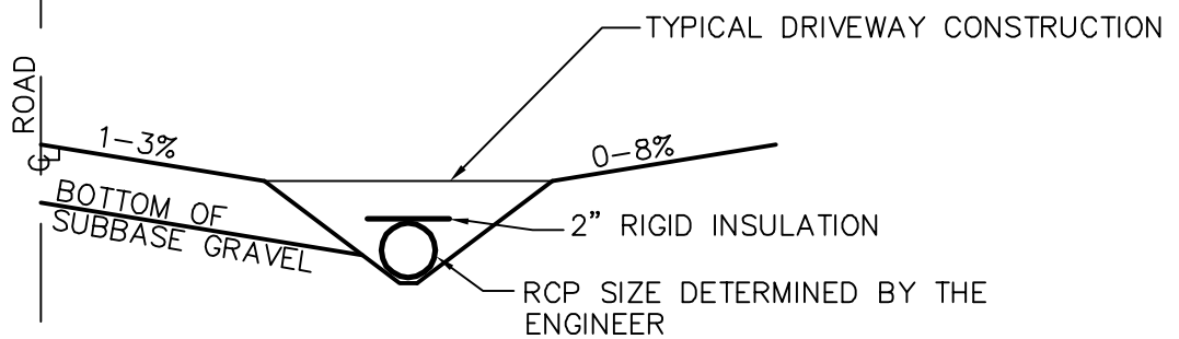
DRIVEWAY CULVERT CROSS SECTION
