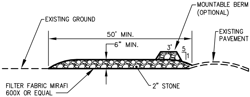
SECTION VIEW
